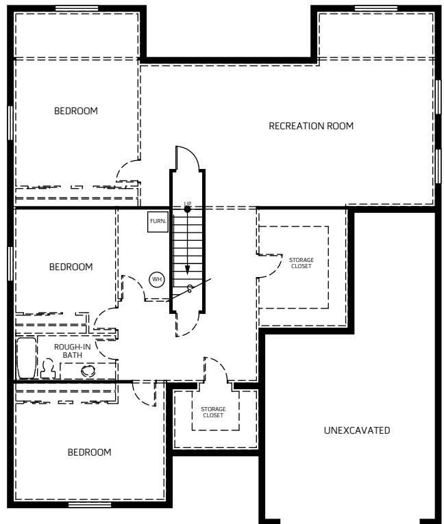
BASEMENT PLAN 2,014 Sq.ft.
