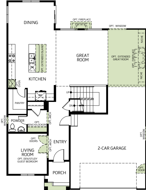
FIRST FLOOR PLAN 1,118 Sq. Ft.
