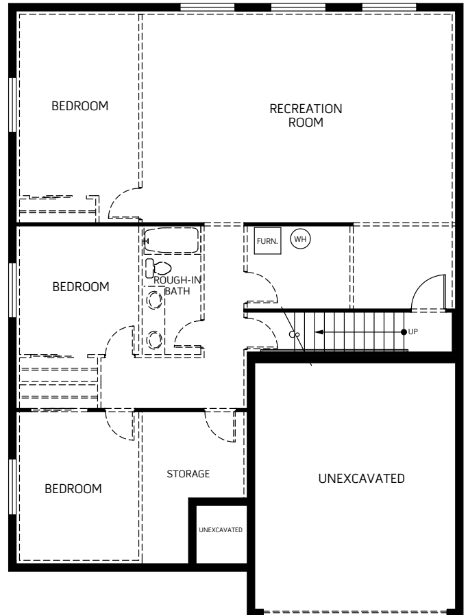
BASEMENT PLAN 25 Sq. Ft. Finished 1,440 Sq. Ft. Unfinished
