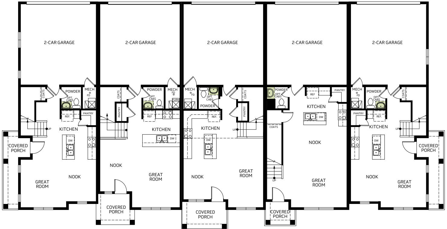
FIRST FLOOR 597 Sq. Ft.
