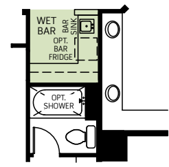
OPTIONAL MASTER WET BAR ILO STORAGE
