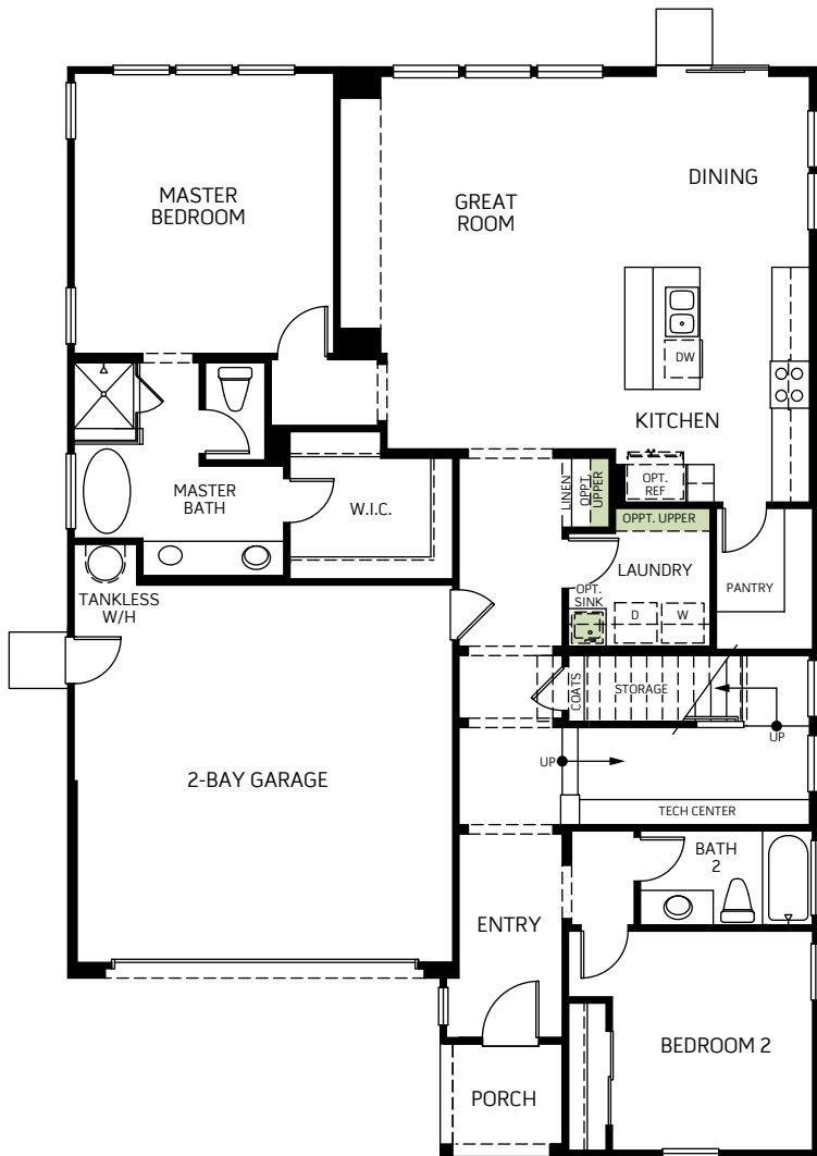
FIRST FLOOR
