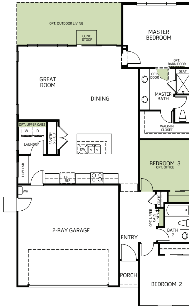
FLOOR PLAN
