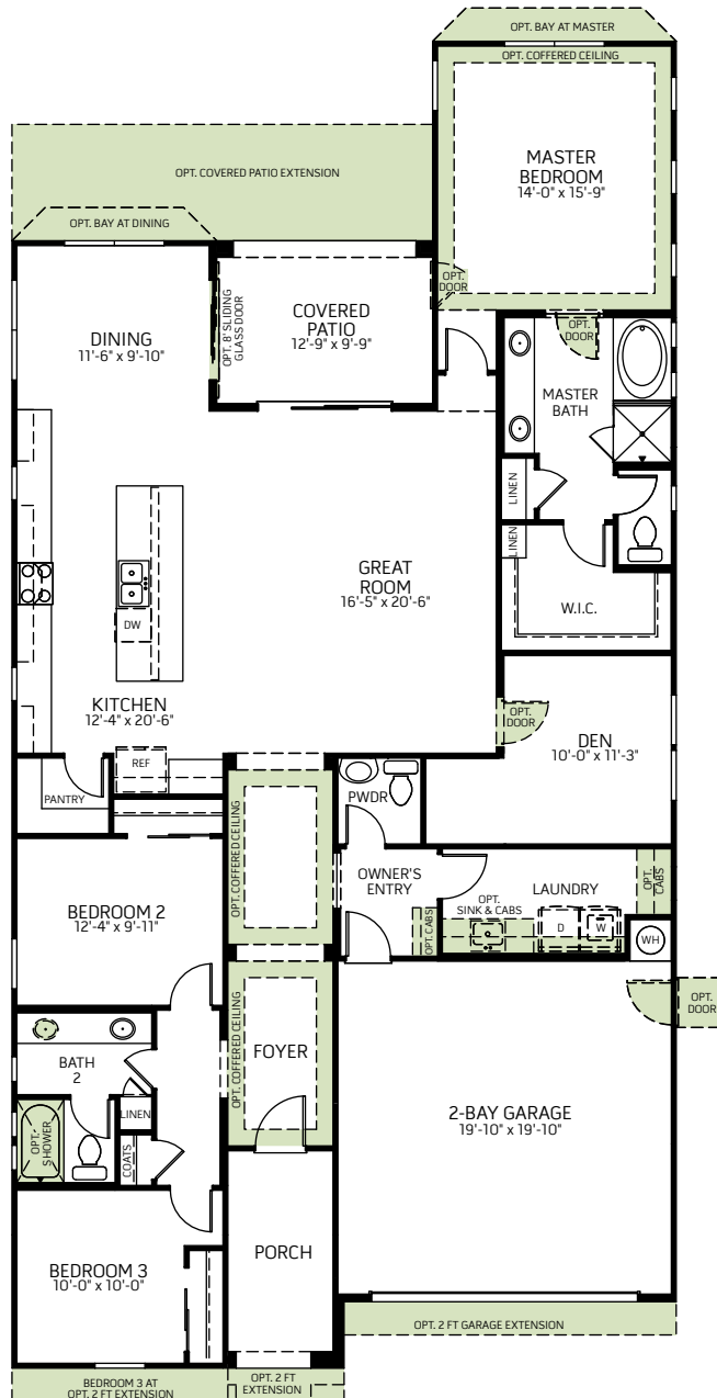
FLOOR PLAN
