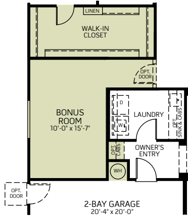
OPTIONAL BONUS ROOM ILO TANDEM GARAGE
