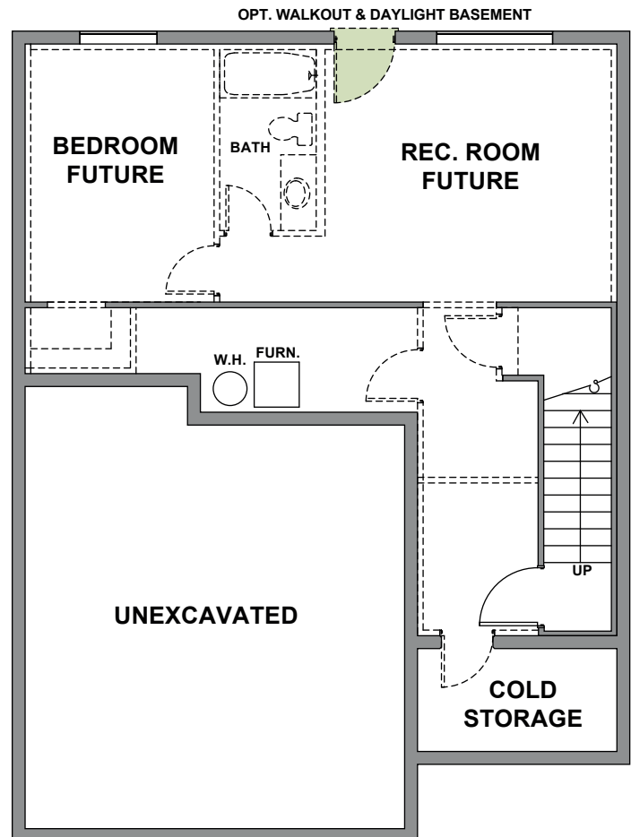
BASEMENT FLOOR PLAN 72 Sq.Ft. Finished 585 Sq.Ft. Unfinished
