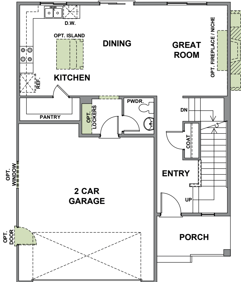
FIRST FLOOR PLAN 739 Sq.Ft.
