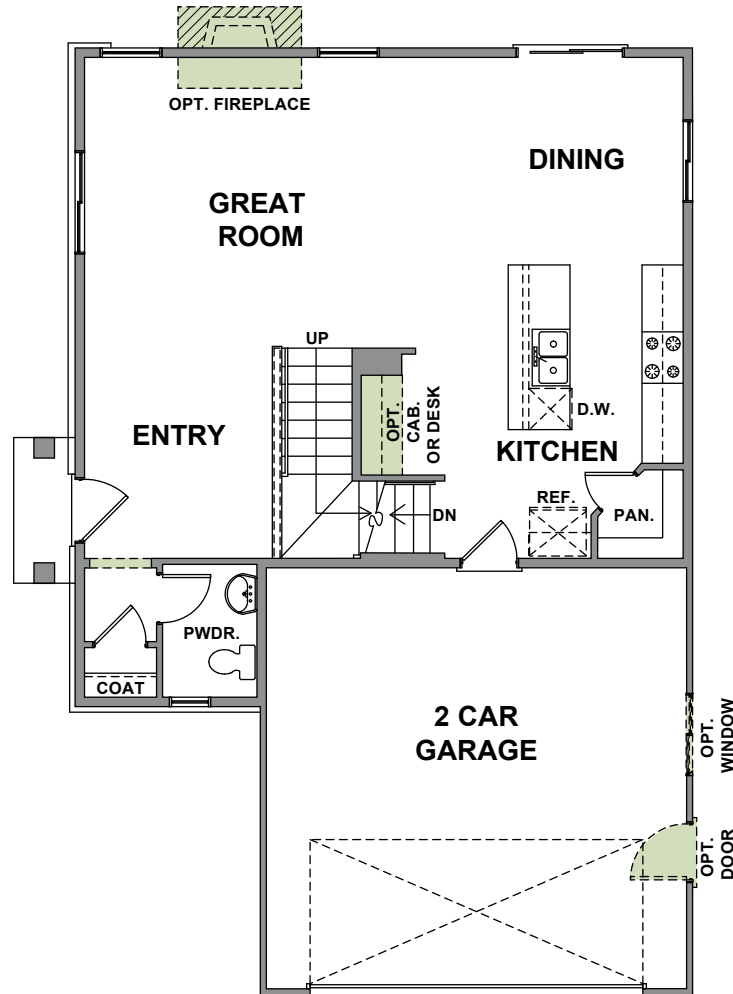
FIRST FLOOR PLAN 821 Sq.Ft.
