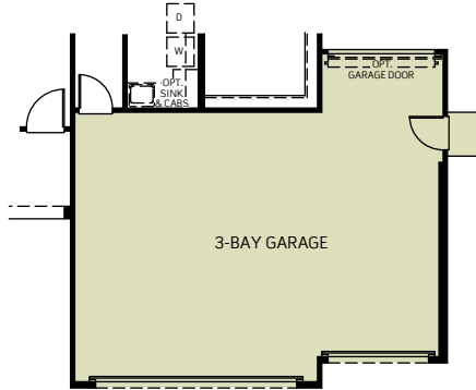
OPTIONAL 3 BAY GARAGE
