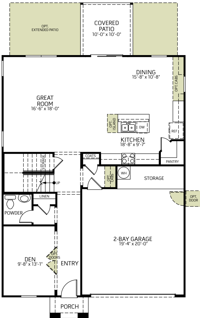
FIRST FLOOR
