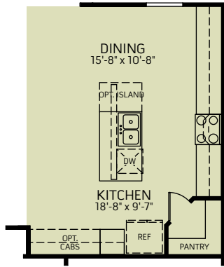
OPTIONAL KITCHEN
