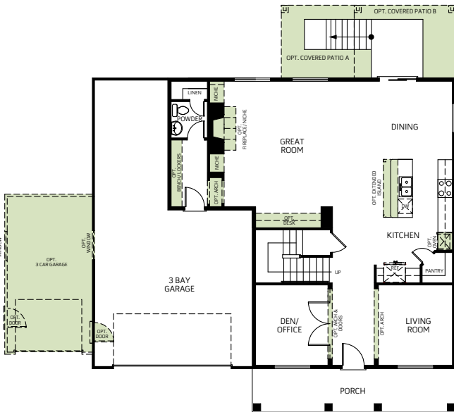
FIRST FLOOR 1,327 Sq. Ft.
