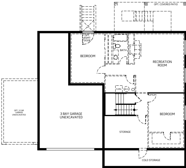
BASEMENT 1,227 Sq. Ft. Unfinished
