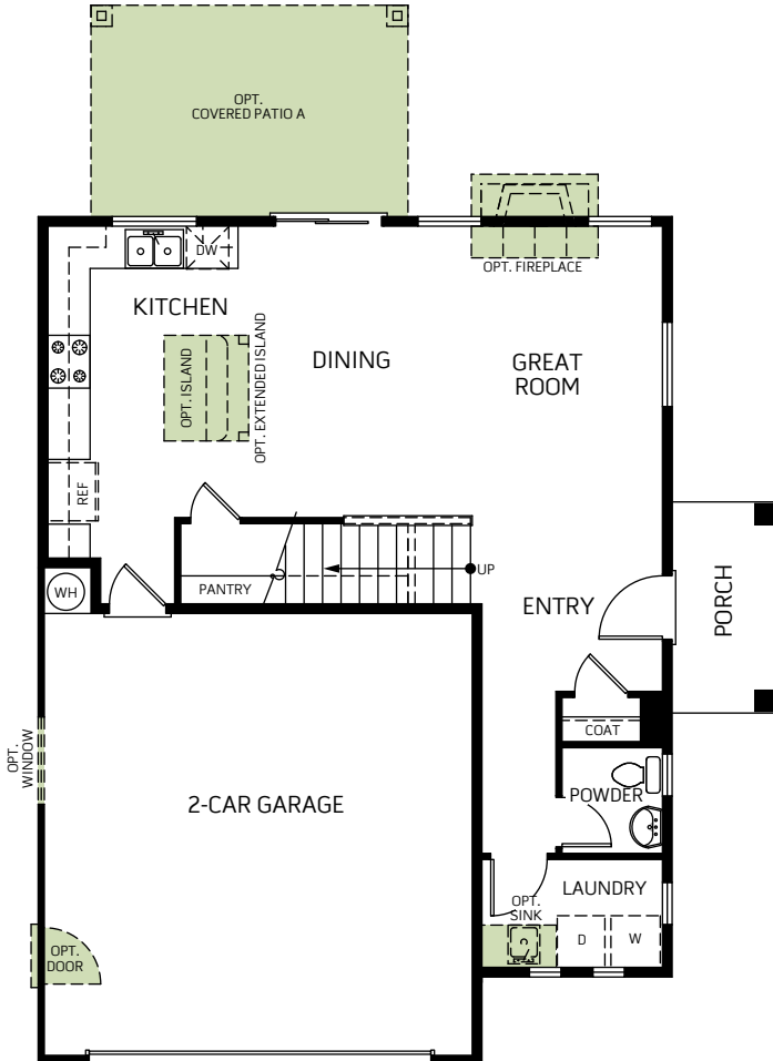
FIRST FLOOR PLAN 727 Sq. Ft.
