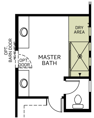
OPTIONAL EXTENDED SHOWER WITH HALF WALL AND GLASS
